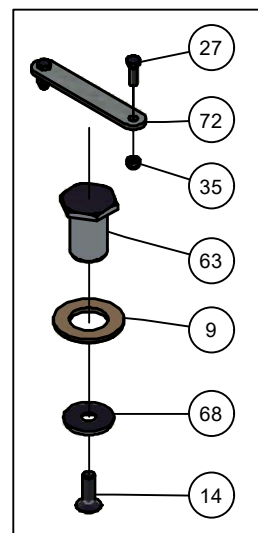
Detail B
