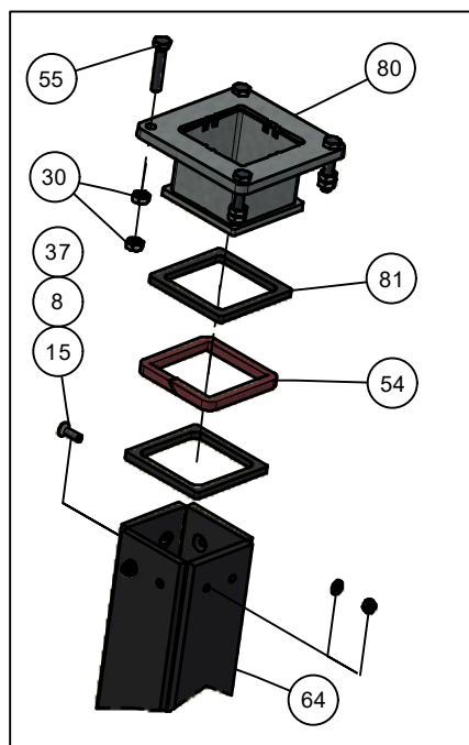
Detail A
